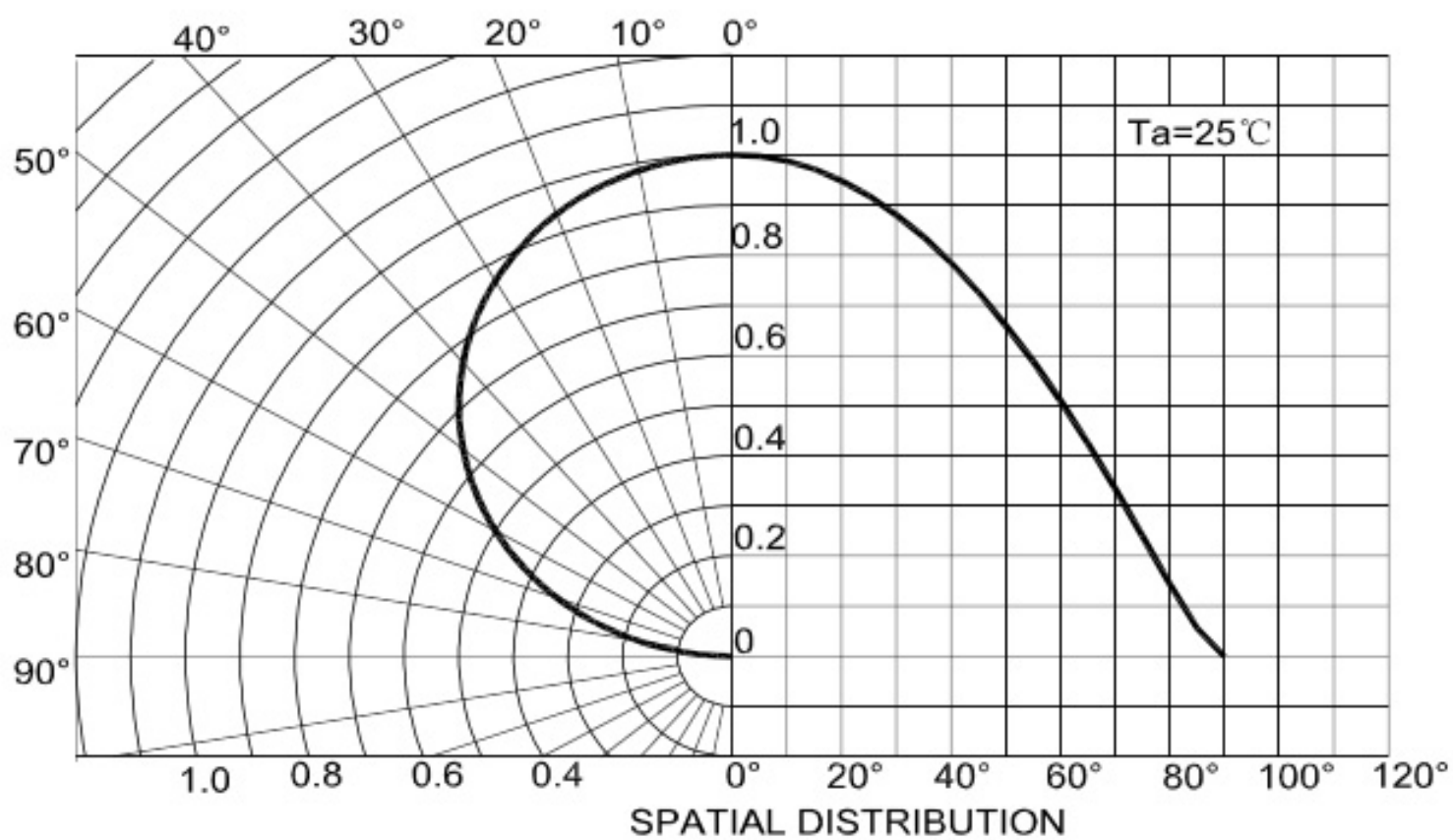
Radiation diagram
